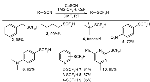
Scheme 2. Cu-mediated difluoromethylation of organothiocyanates. Reaction conditions: 1.0 mmol of organothiocyanate, 1.0 mmol of CuSCN, 4.0 mmol of CsF, 2.0 mmol of \text{TMS}-\text{CF}_2\text{H} in 2 mL of DMF, 12 h, RT. Yields are of isolated products. [a] Yields determined by ^{19}\text{F} NMR spectroscopy using trifluoroethanol as an internal standard.
